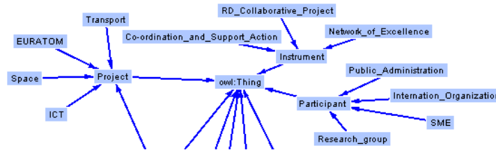
Figure 2: a fragment of the European Projects Ontology.
