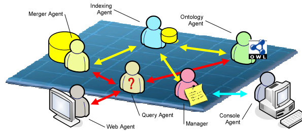
Figure 1: the agent roles in AgentSeeker.
